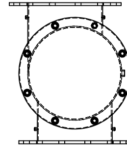
LEFT SIDE TANGENT DISCHARGE
